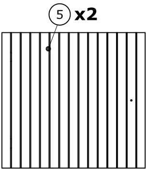
498x470x16 mm
